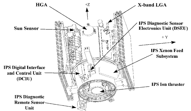
Fig. 1 New Millennium DS1 in the stowed configuration showing the location of the IPS components.
