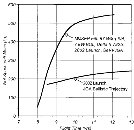
Fig. 2 SEP performance for the Pluto Flyby mission relative to ballistic Jupiter Gravity Assist trajectories using conventional chemical propulsion.
